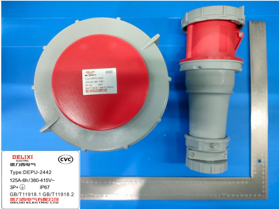
DEPU-2442 125A-6h/415V~3P+PE IP67
