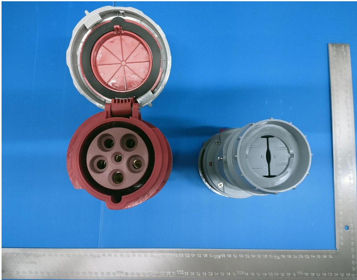
DEPU-2452 125A-6h/415V~3P+N+PE IP67
