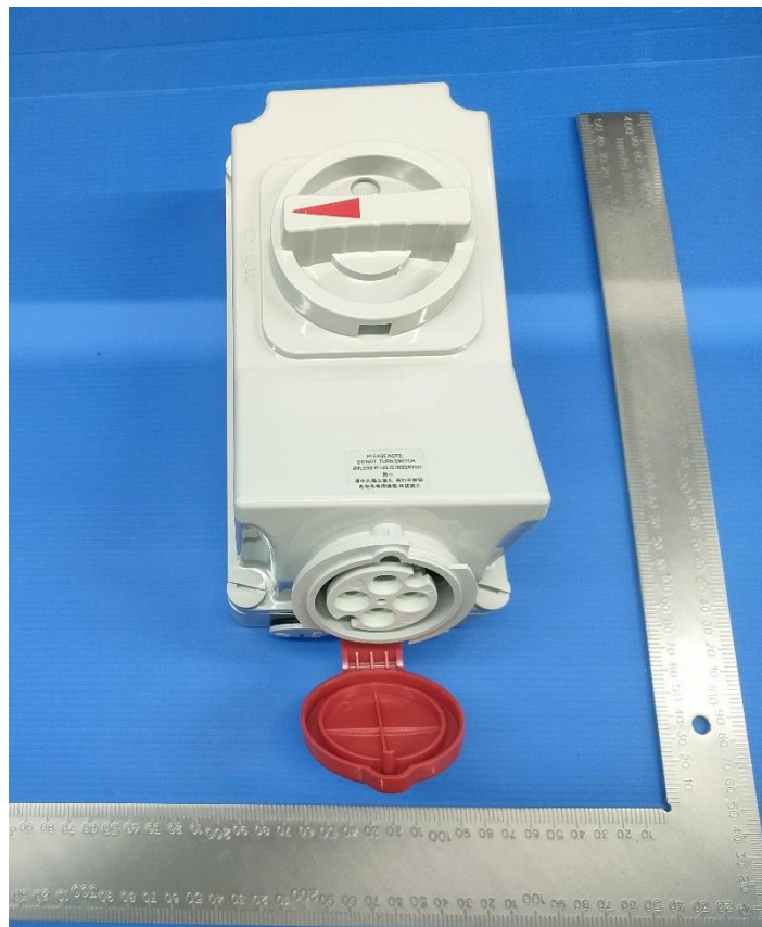
DEPU-614 16A-6h/415V~3P+PE IP44
