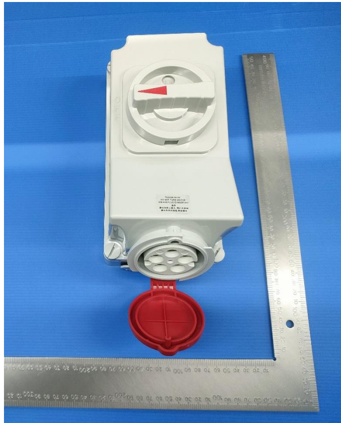
DEPU-615 16A-6h/415V~3P+N+PE IP44
