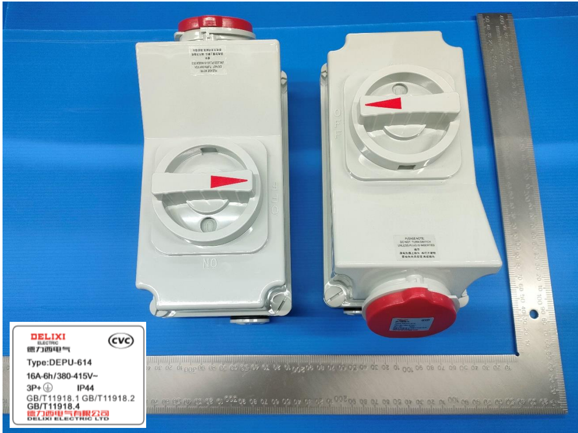
DEPU-614 16A-6h/415V~3P+PE IP44
