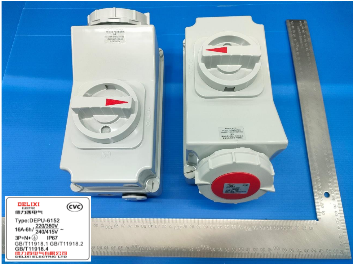
DEPU-6152 16A-6h/415V~3P+N+PE IP67
