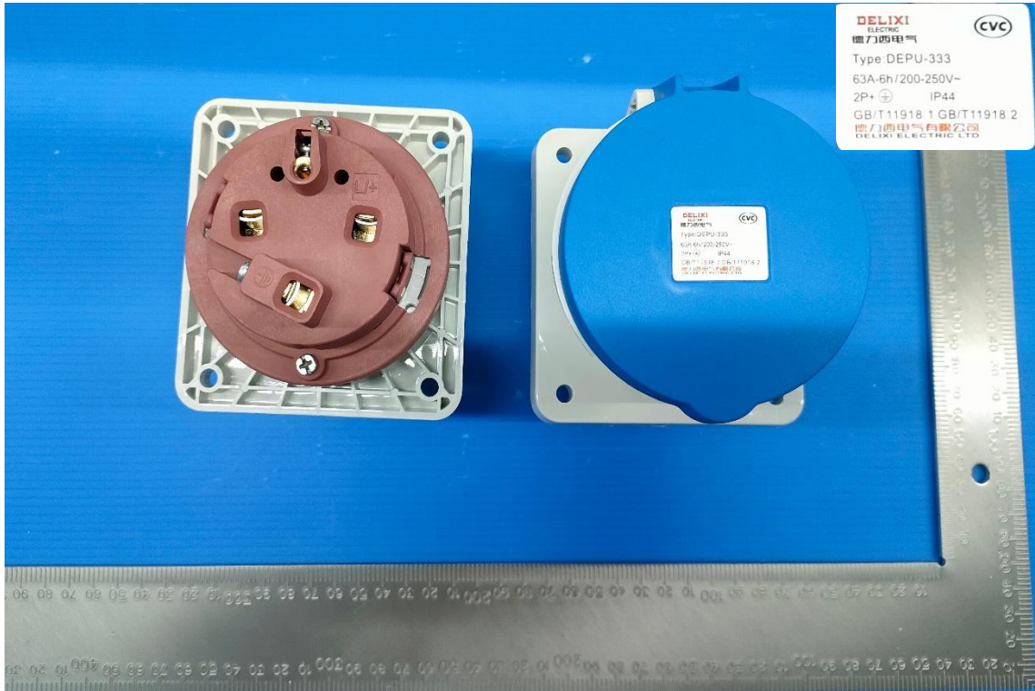
DEPU-333 63A-6h/250V ~ 2P+PE IP44
