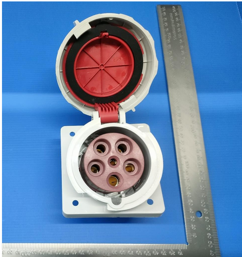
DEPU-4352 63A-6h/415V~3P+N+PE IP67
