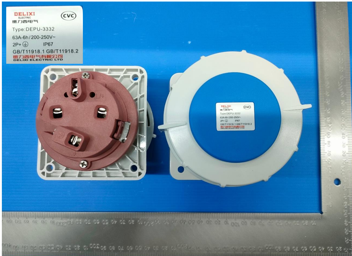
DEPU-3332 63A-6h/250V ~ 2P+PE IP67
