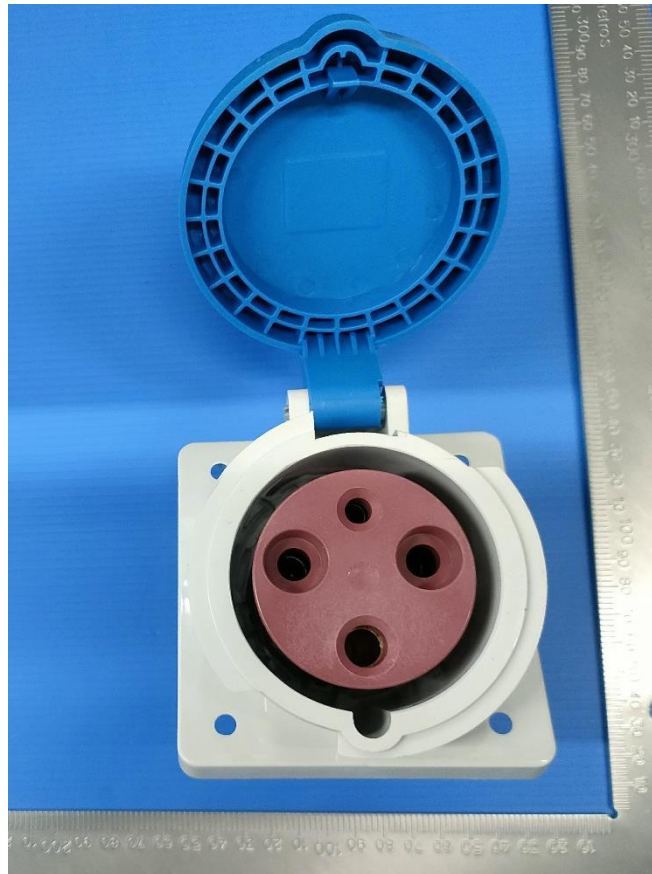
DEPU-433 63A-6h/250V ~ 2P+PE IP44
