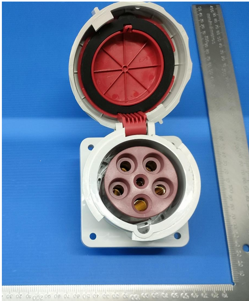
DEPU-3352 63A-6h/415V~3P+N+PE IP67
