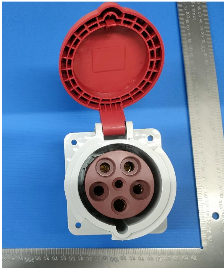
DEPU-335 63A-6h/415V ~ 3P+N+PE IP44
