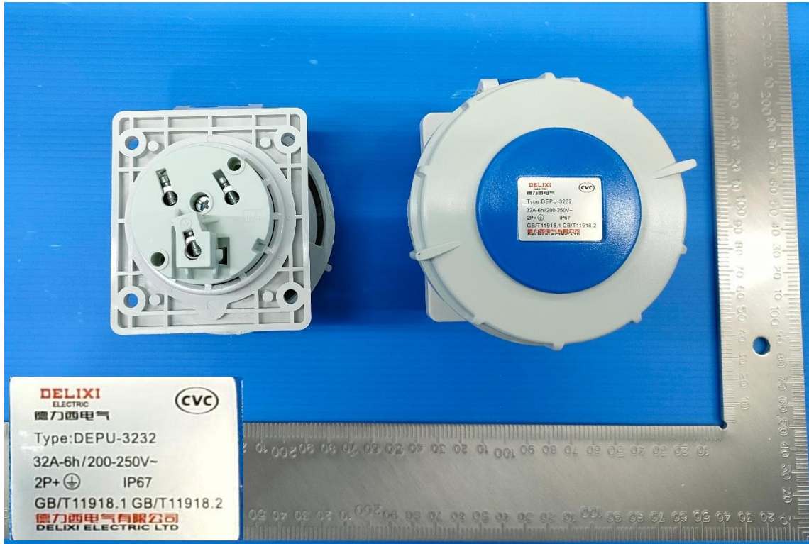
DEPU-3232 32A-6h/250V ~ 2P+PE IP67
