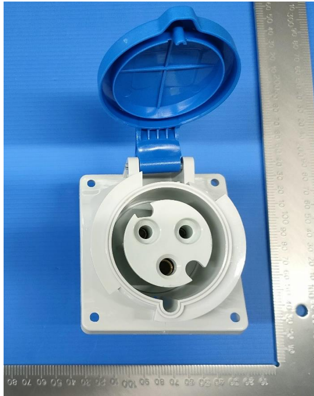
DEPU-423 32A-6h/250V ~ 2P+PE IP44
