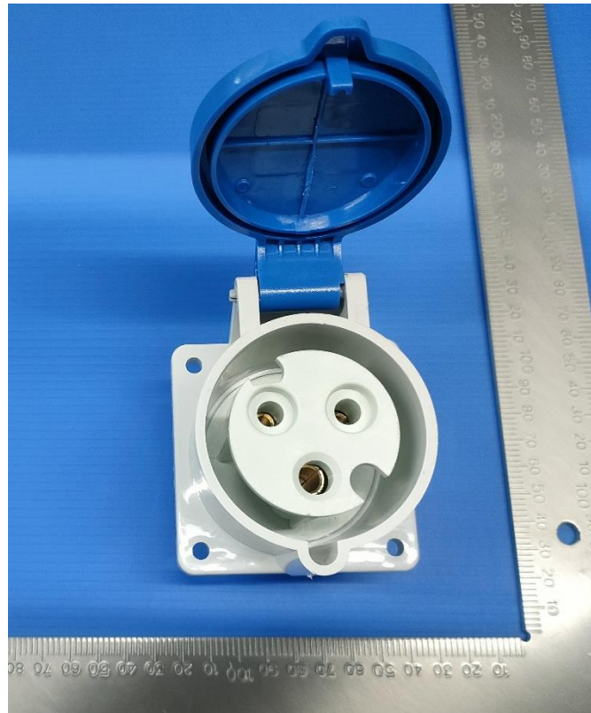
DEPU-323 32A-6h/250V ~ 2P+PE IP44
