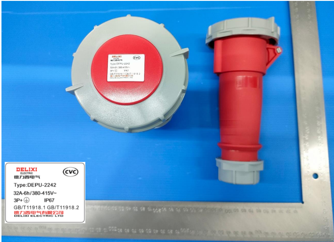
DEPU-2242 32A-6h/415V~3P+PE IP67
