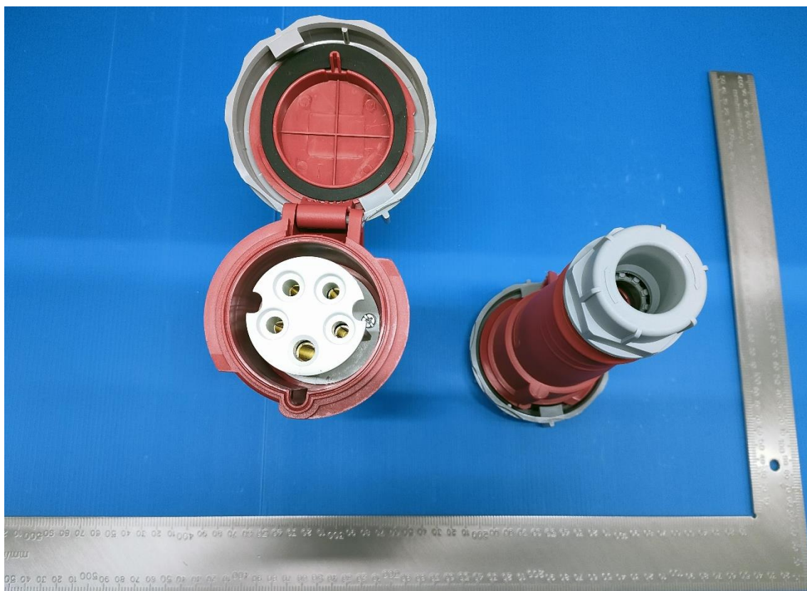
DEPU-2252 32A-6h/415V~3P+N+PE IP67
