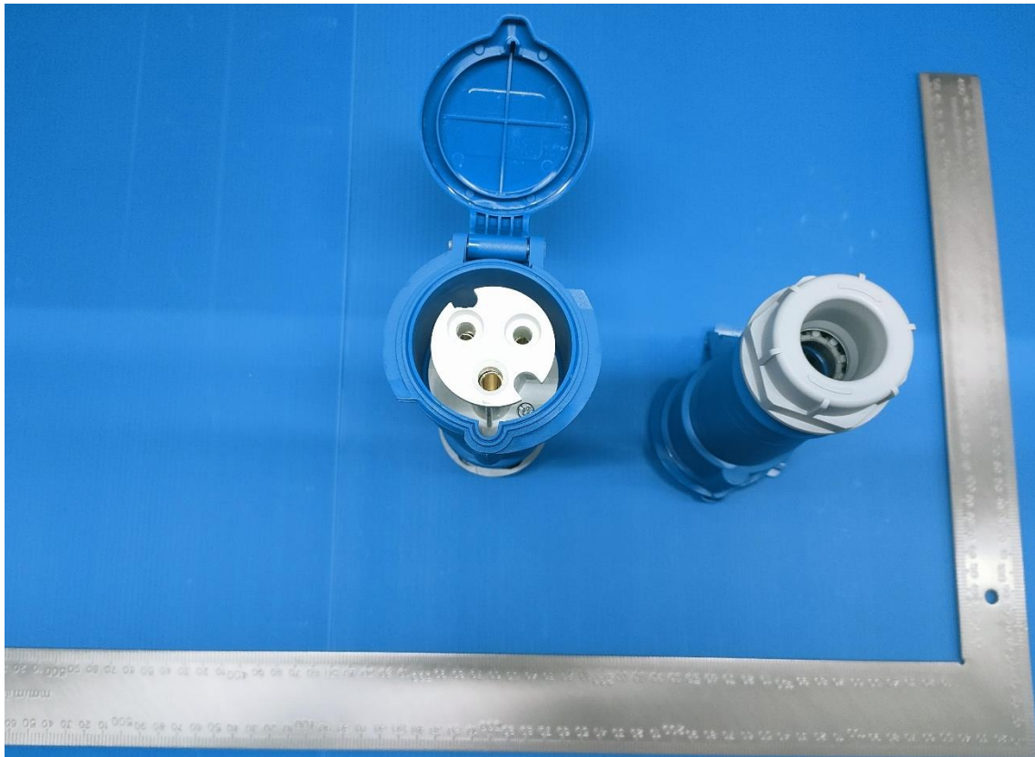
DEPU-223 32A-6h/250V~2P+PE IP44
