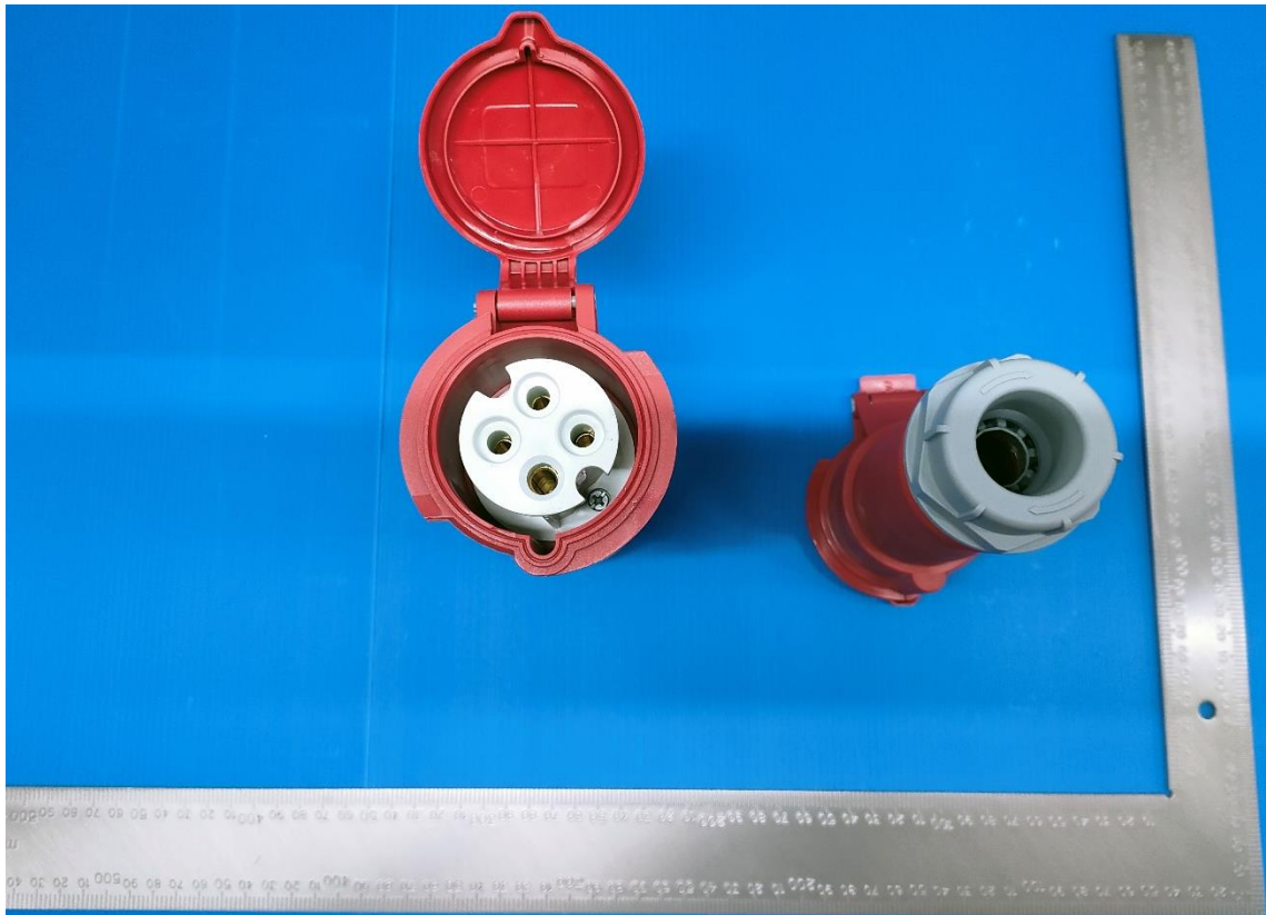
DEPU-224 32A-6h/415V~3P+PE IP44
