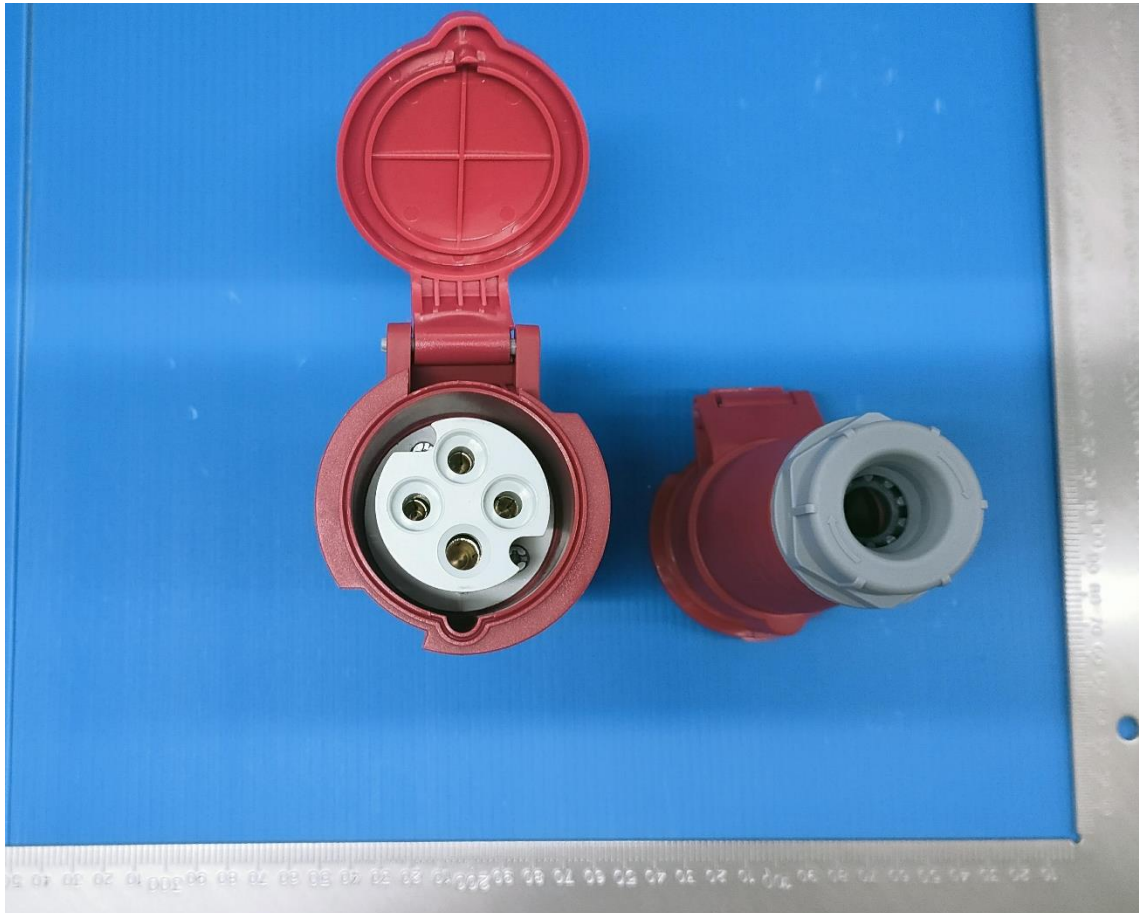
DEPU-214 16A-6h/415V~3P+PE IP44
