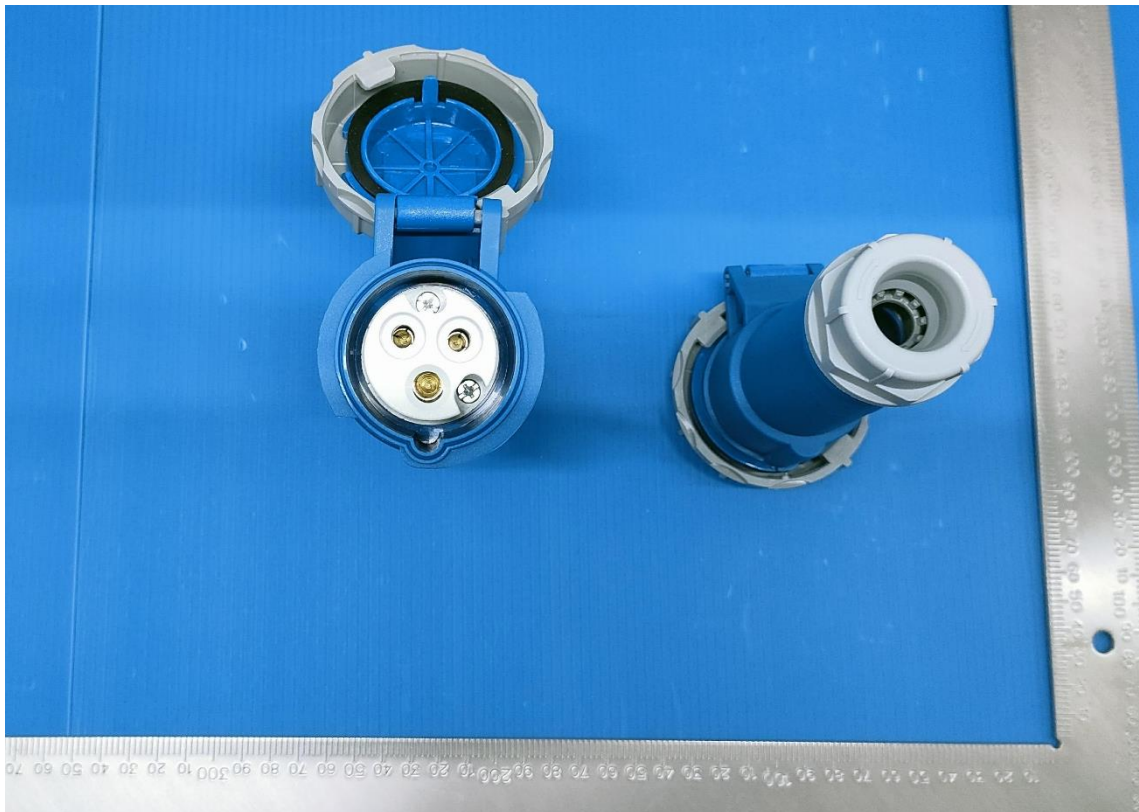
DEPU-2132 16A-6h/250V~2P+PE IP67
