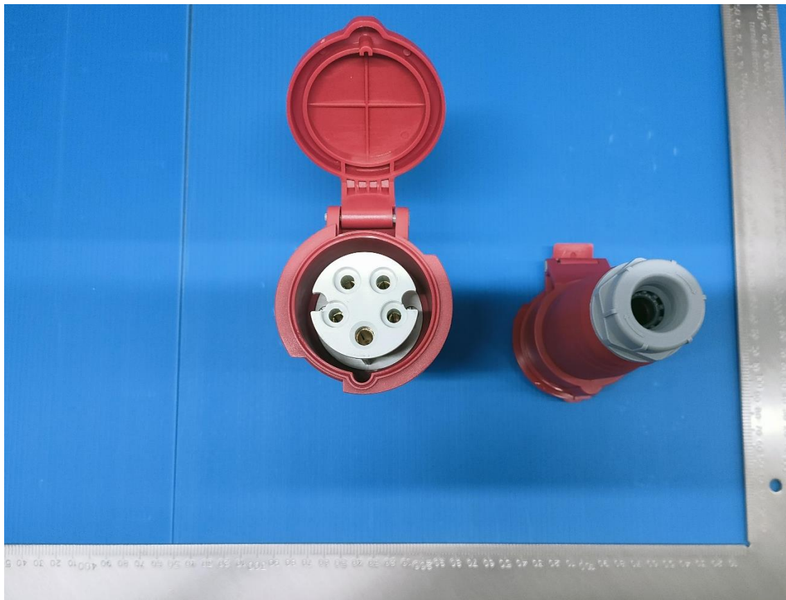
DEPU-215 16A-6h/415V~3P+N+PE IP44
