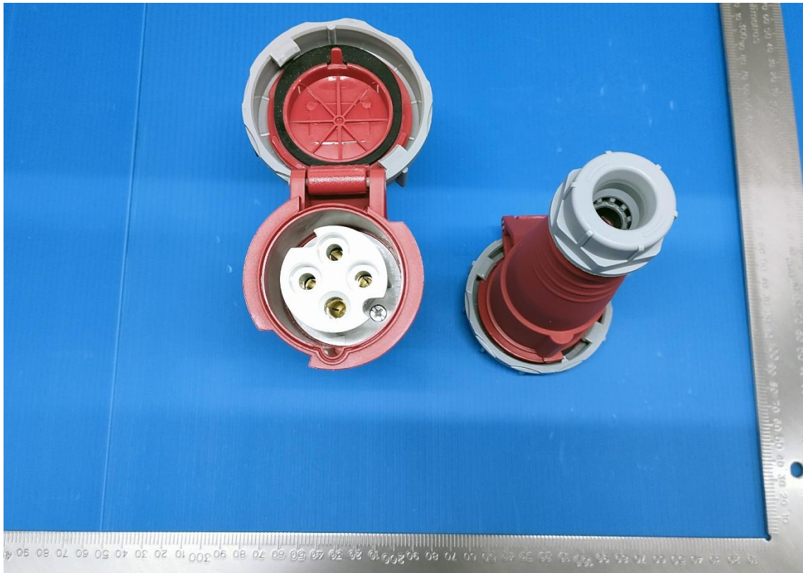
DEPU-2142 16A-6h/415V~3P+PE IP67
