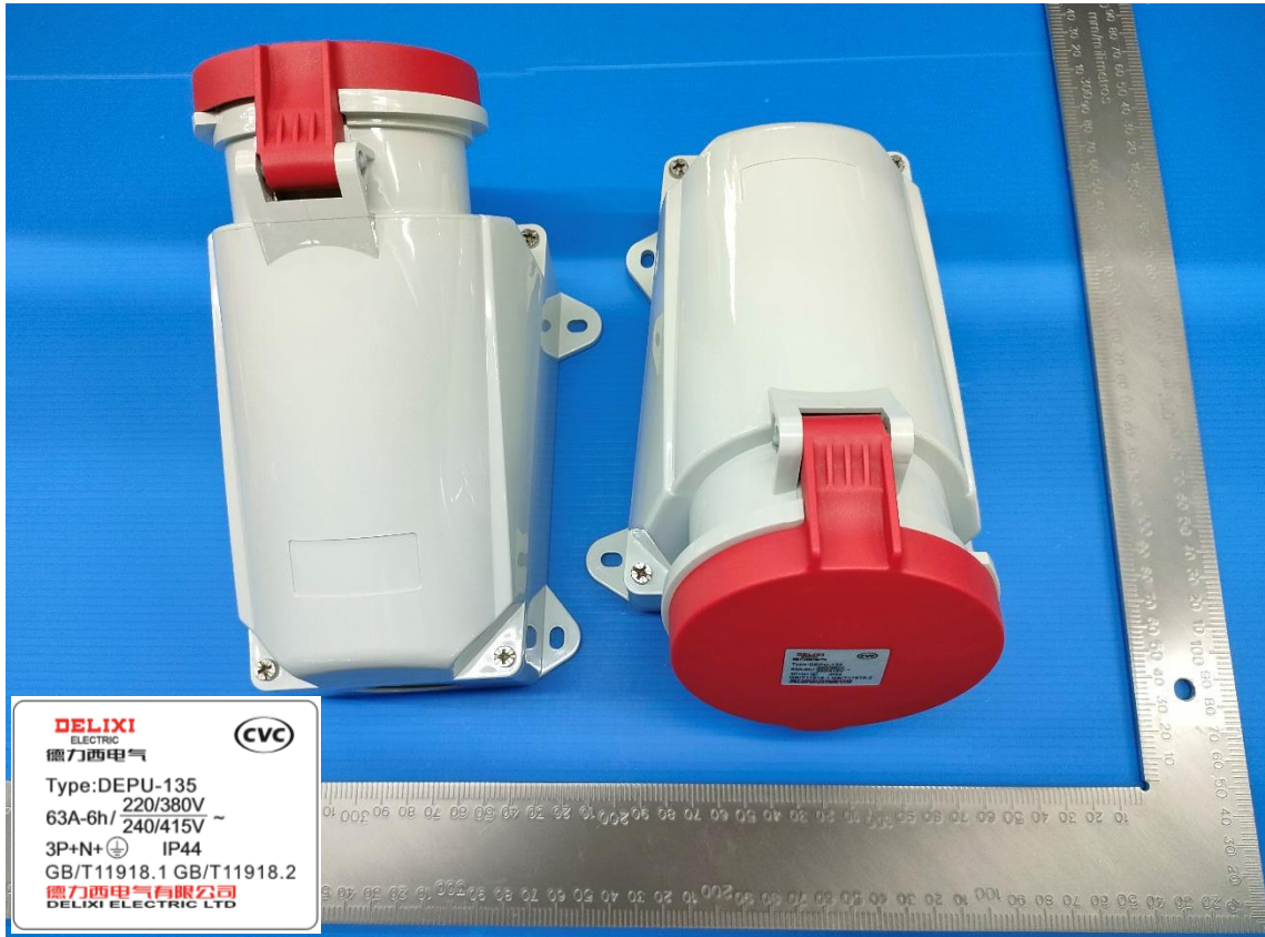
DEPU-135 63A-6h/415V ~ 3P+N+PE IP44
