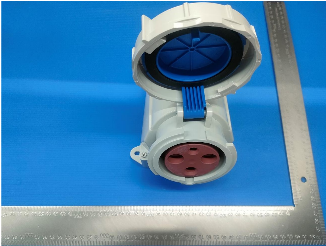
DEPU-1332 63A-6h/250V ~ 2P+PE IP67
