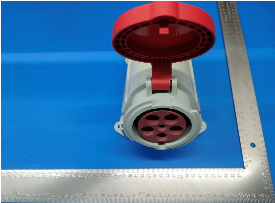
DEPU-135 63A-6h/415V ~ 3P+N+PE IP44
