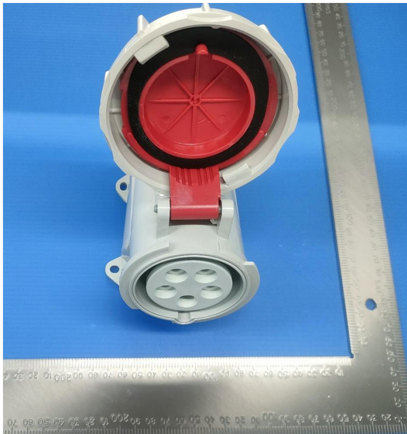
DEPU-1152 16A-6h/415V ~ 3P+N+PE IP67
