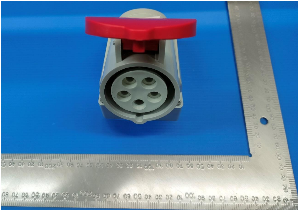
DEPU-115 16A-6h/415V ~ 3P+N+PE IP44
