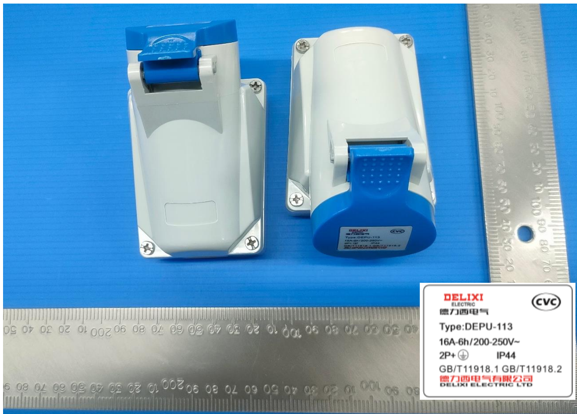
DEPU-113 16A-6h/250V ~ 2P+PE IP44
