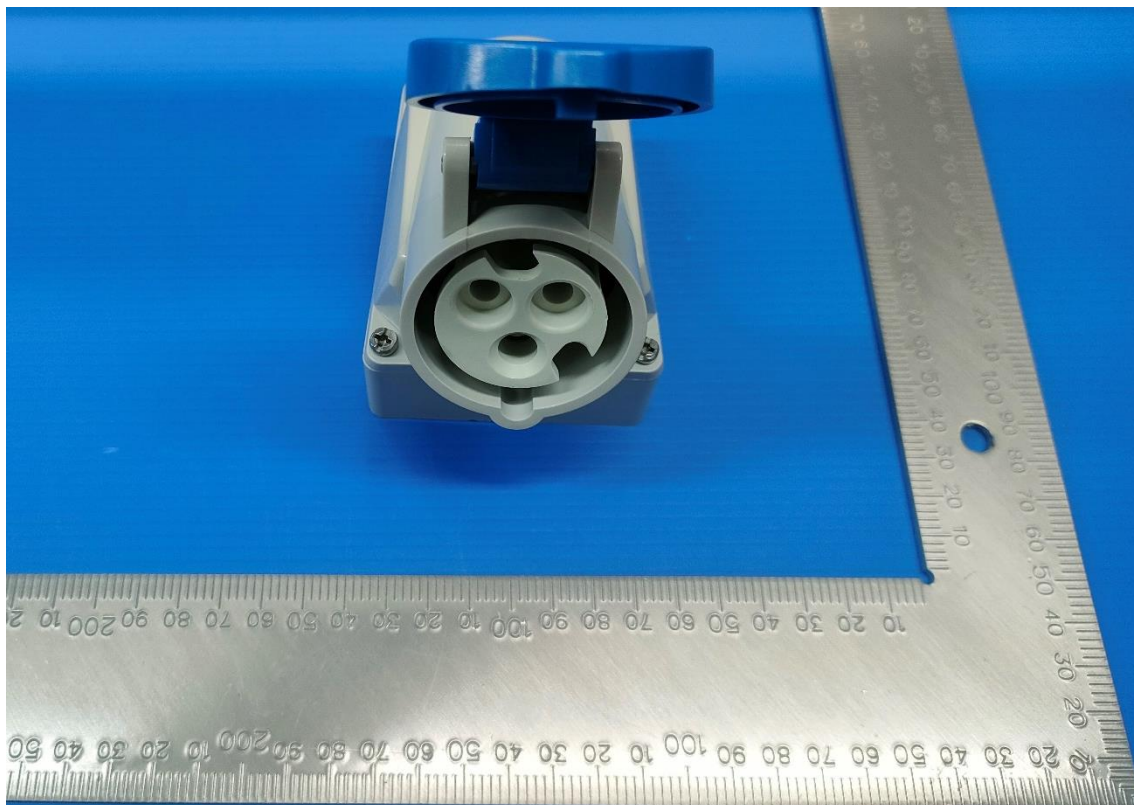
DEPU-113 16A-6h/250V ~ 2P+PE IP44
