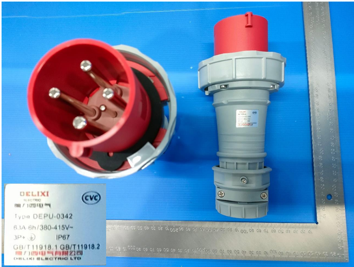
DEPU-0342 63A-6h/415V~3P+PE IP67
