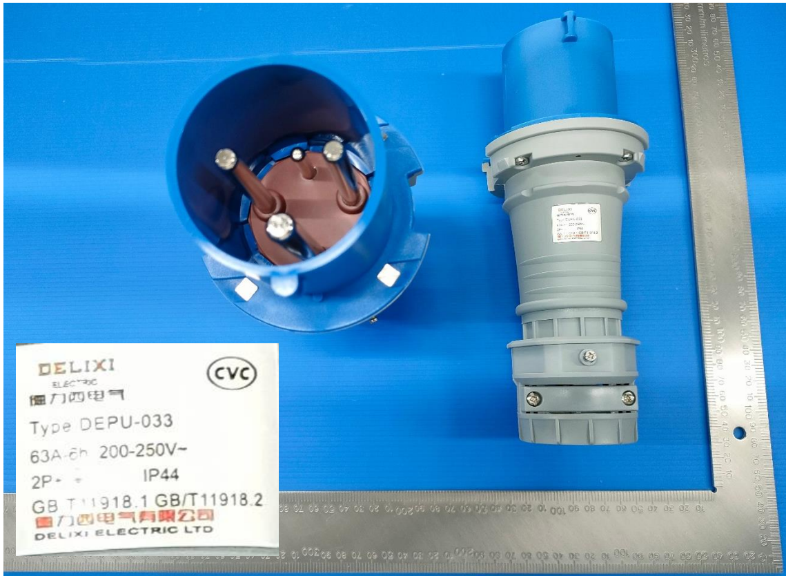
DEPU-033 63A-6h/250V~2P+PE IP44
